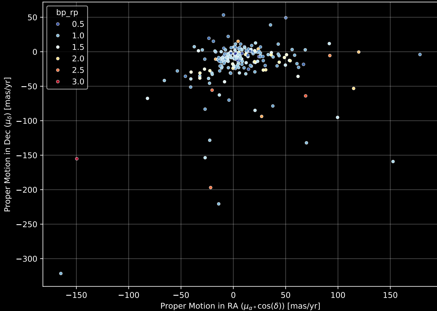
APOGEE DR17 Field: [K2_C3_059-48_btx] Proper Motion Diagram (n= 224)
