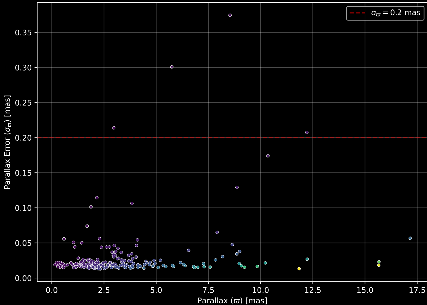
APOGEE DR17 Field: [K2_C3_059-48_btx] Parallax Quality (n= 224)
