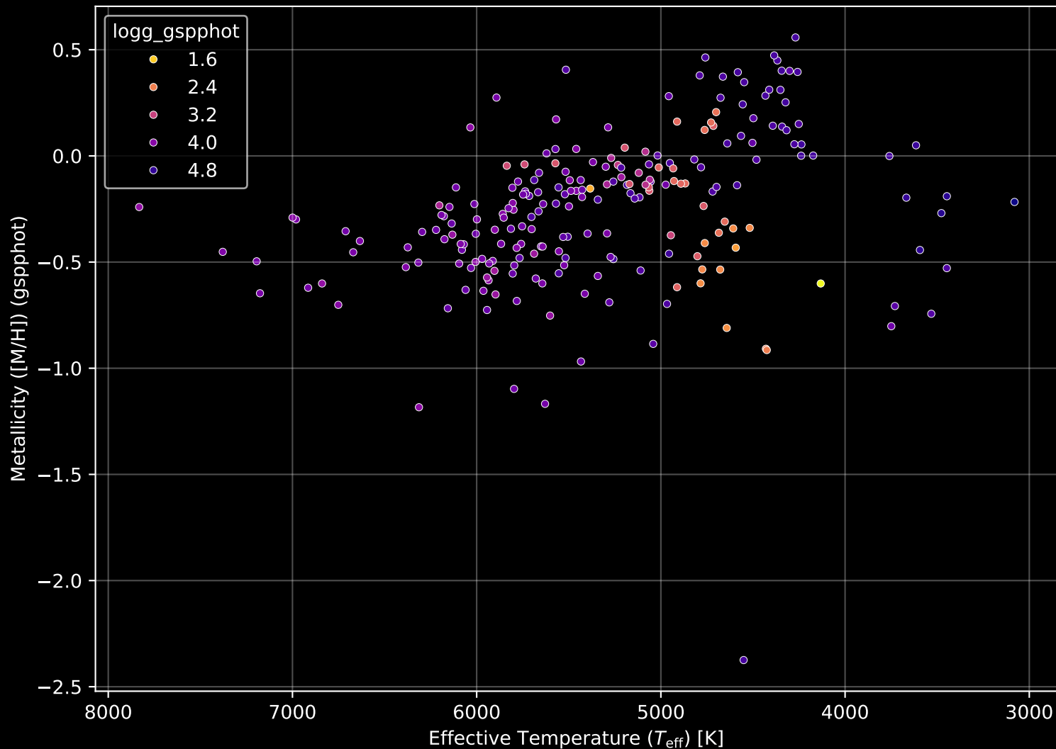
APOGEE DR17 Field: [K2_C3_059-48_btx] Stellar Population Parameters (n= 224)
