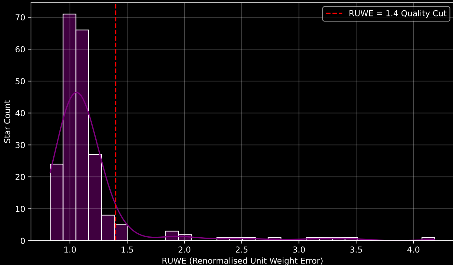
GAPOGEE DR17 Field [K2_C3_059-48_btx] RUWE Distribution (n= 215)
