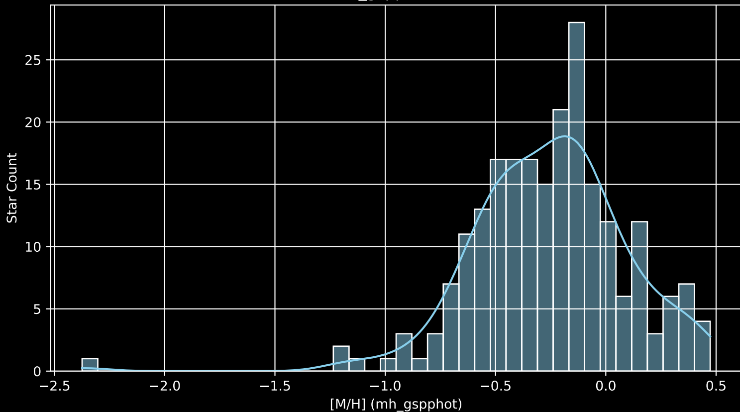
APOGEE DR17 Field: [K2_C3_059-48_btx [M/H] (mh_gspphot) (n= 223)
