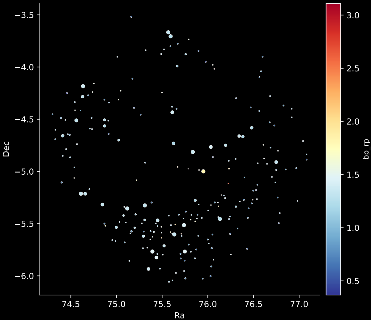
APOGEE DR17 Field: [K2_C3_059-48_btx] Stars: 224
