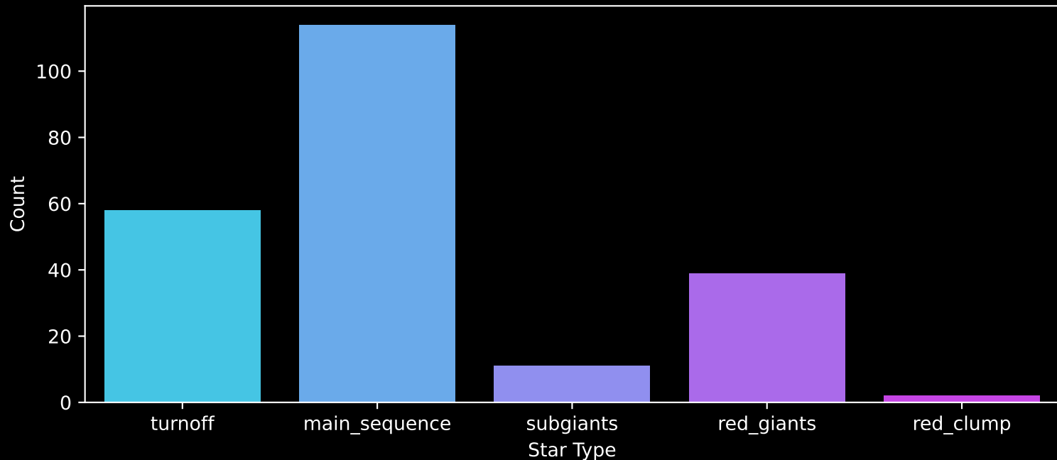
APOGEE DR17 Field: [K2_C3_059-48_btx] Count plot of Star Type
